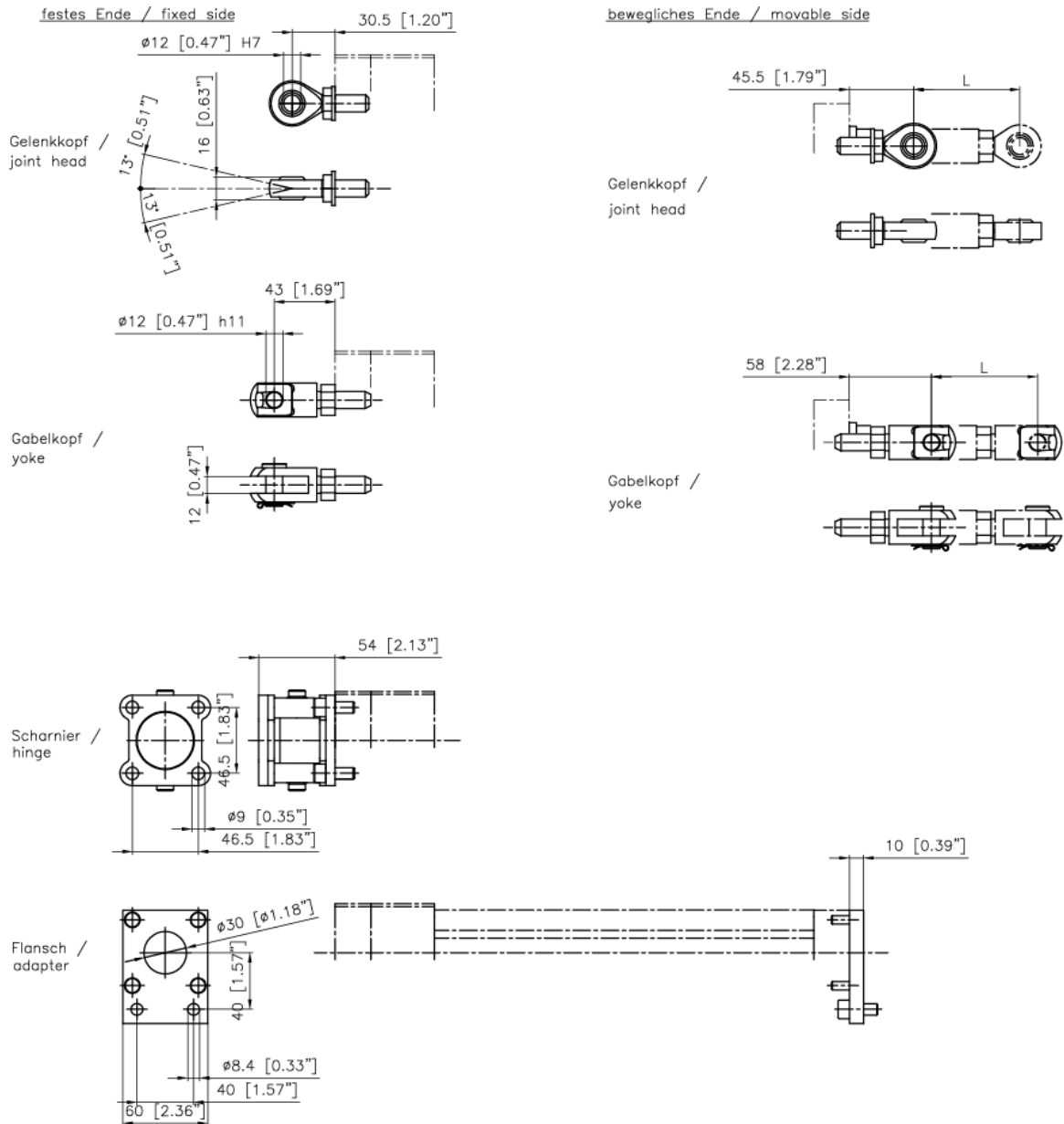
Figure 3: Mounting Accessories
