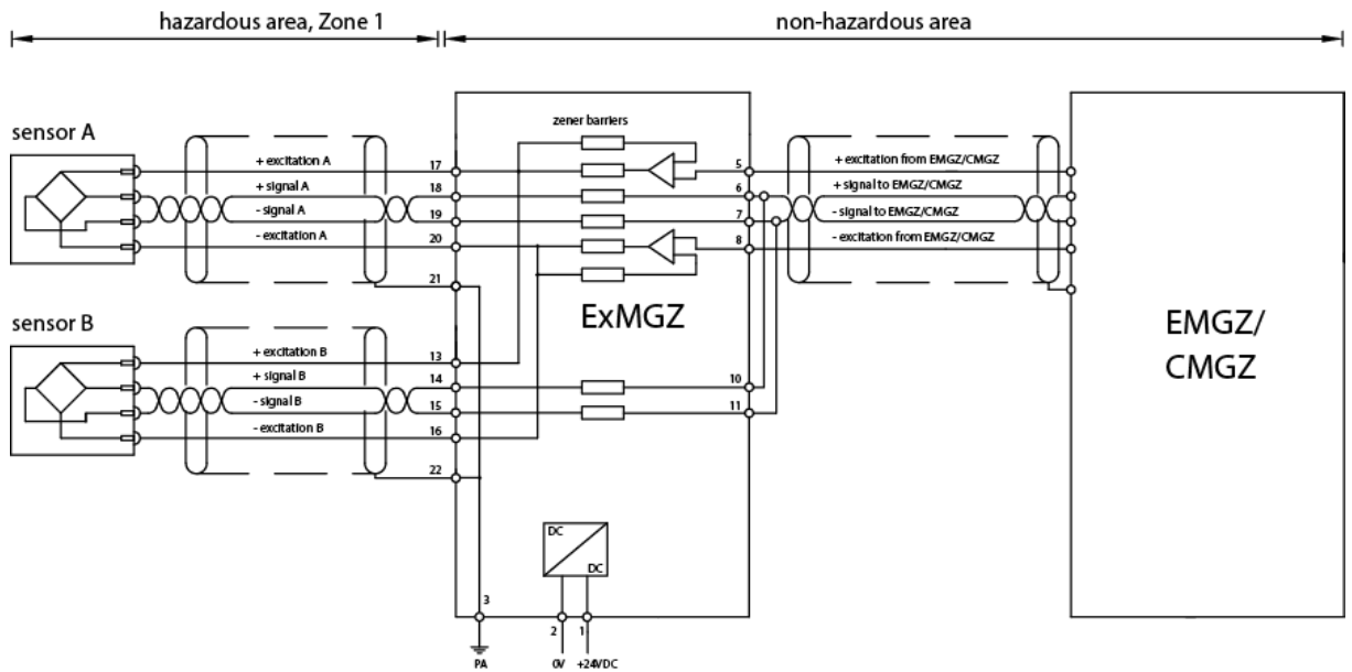
Figure 1: electrical connection single-channel
