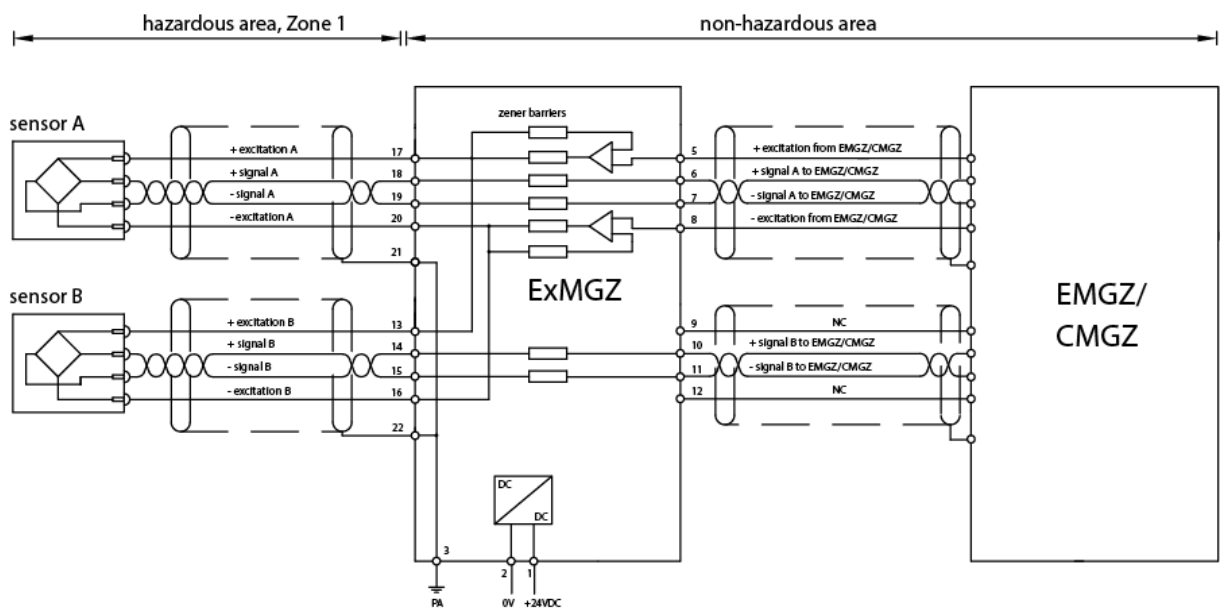
Figure 2: electrical connection dual-channel
